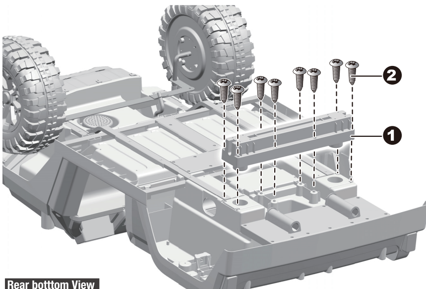
Rear botttom View
